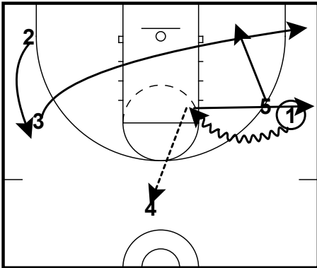
Secondary (Arsenal) Ball Screen Motion
