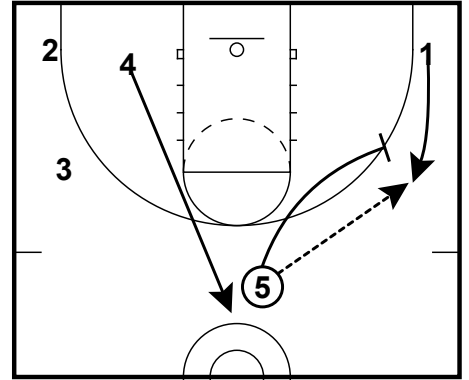
Secondary (Arsenal) Ball Screen Motion
